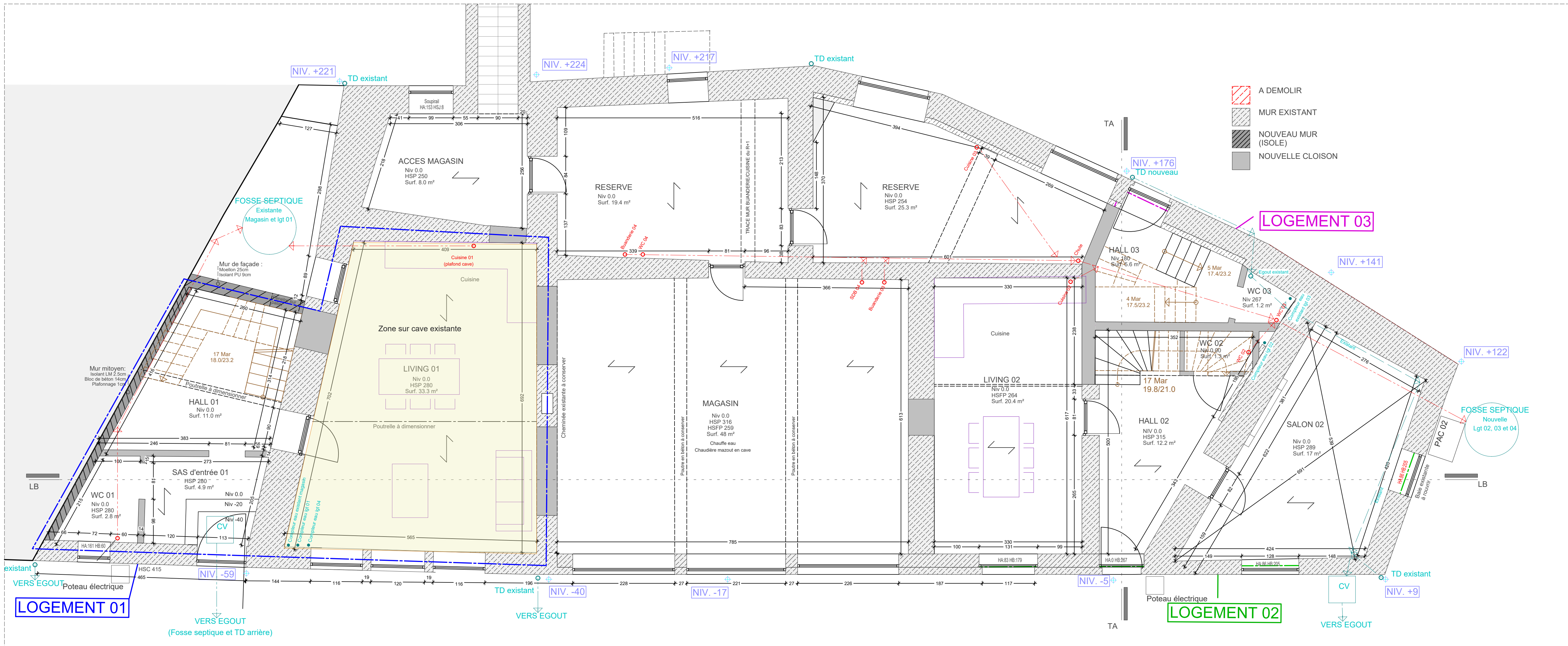
PLAN R0 - 1/50
