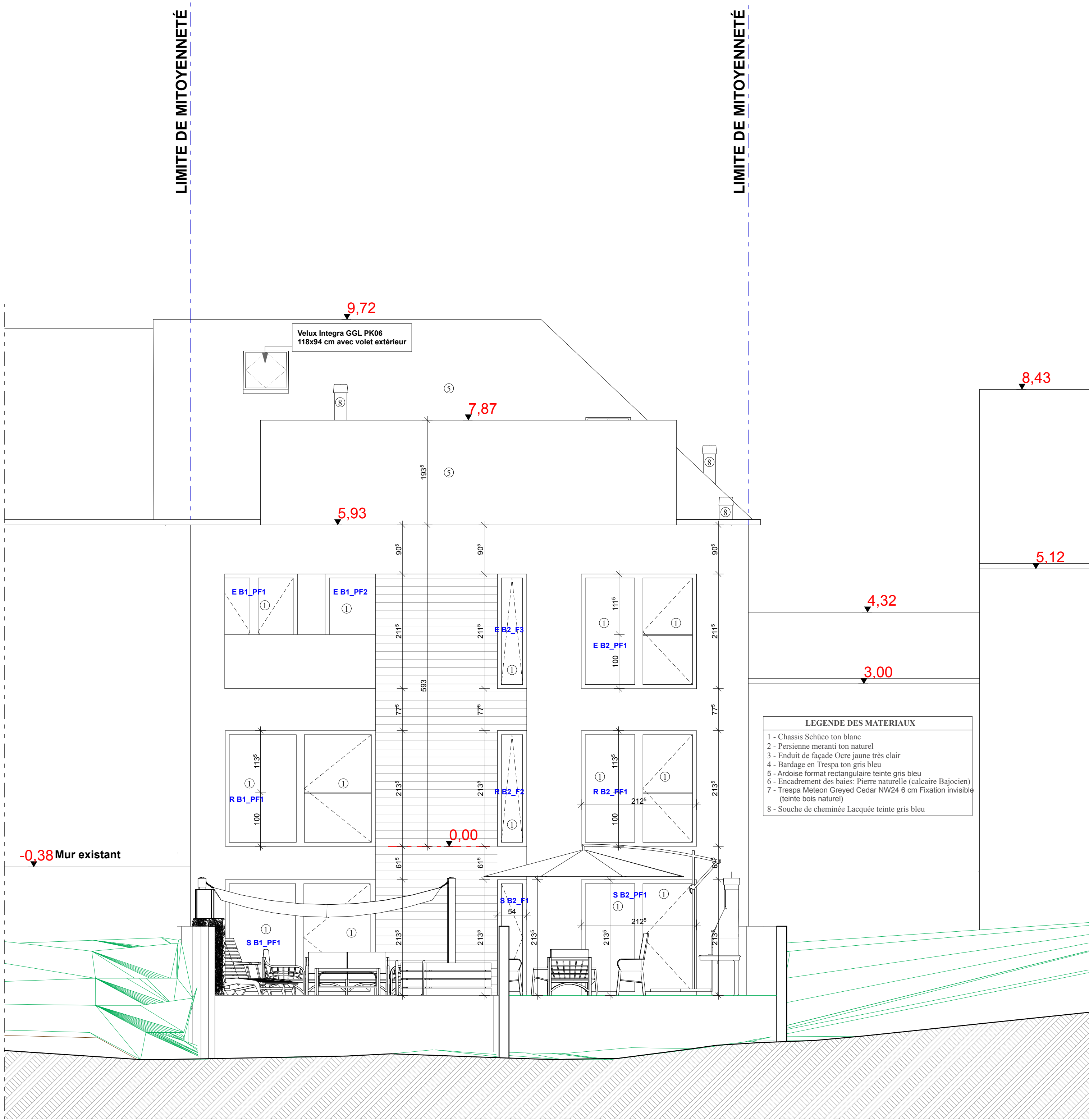
FACADE ARRIERE
